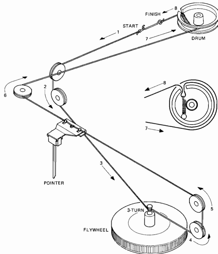
Figure 1. Dial Stringing
